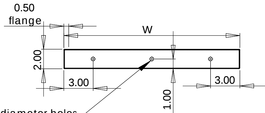
End View [1:6]
