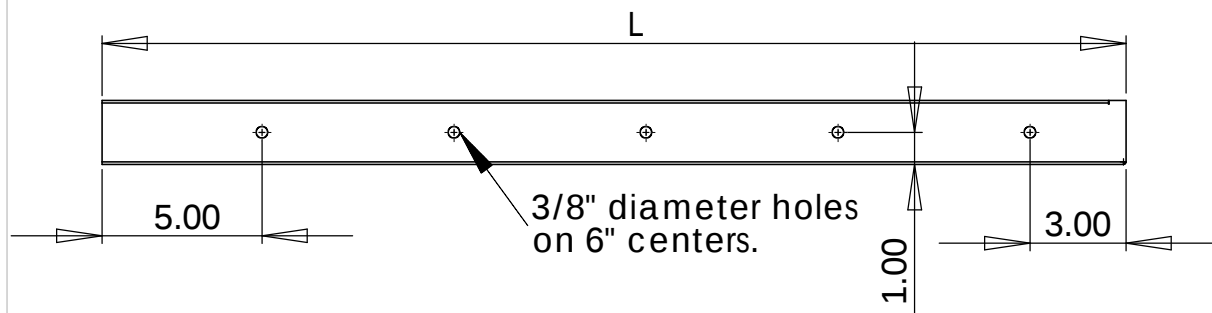
Side Flange View [1:6]
