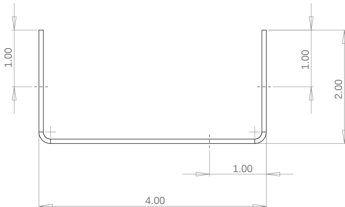
Profile [1:1]
