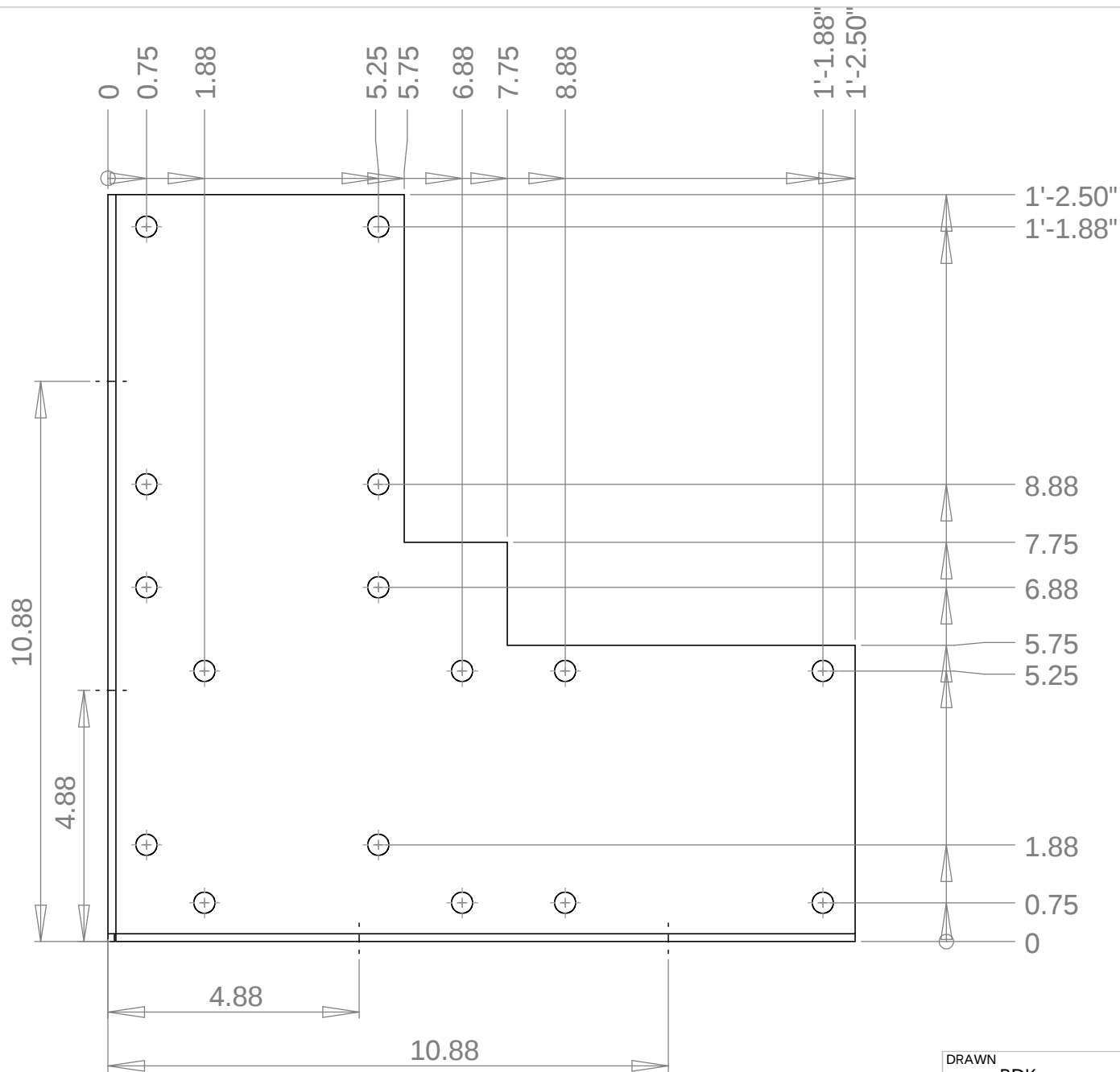
Bottom View
