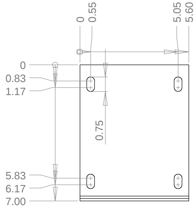
Side View [1:3]
