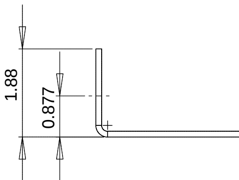
Flange View [1:2]
