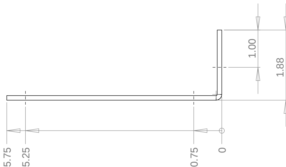
Profile [2:3]
