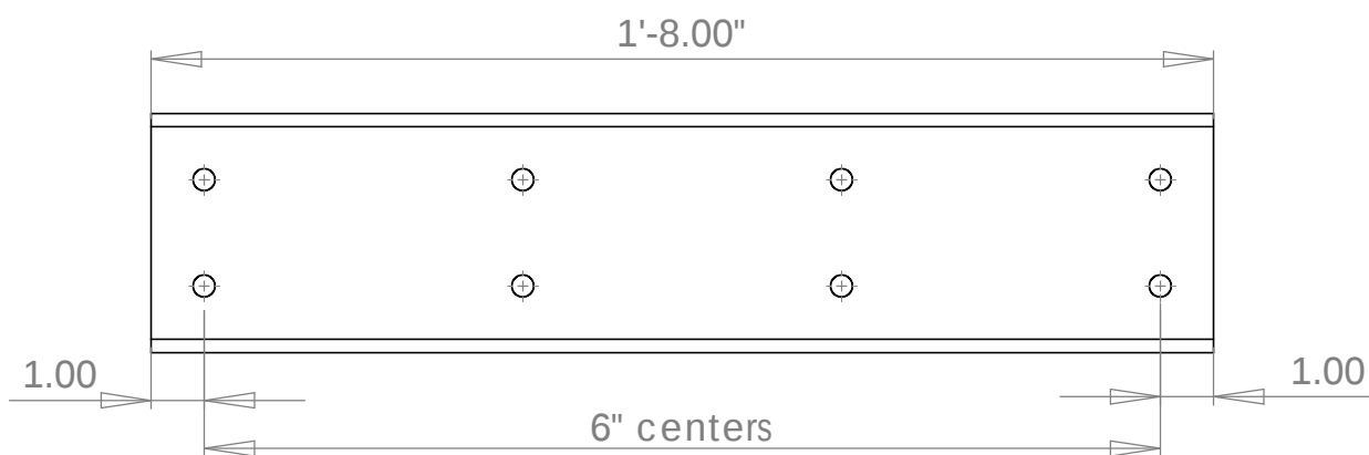
Bottom View
