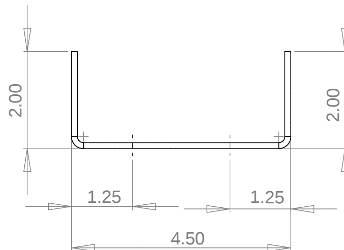
Side View [1:2]
