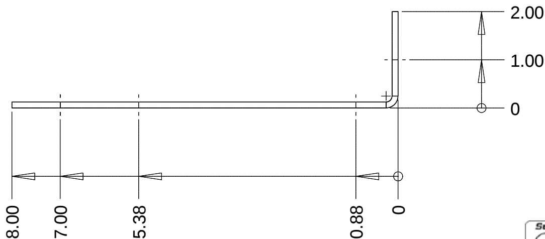
Profile [1:2]
