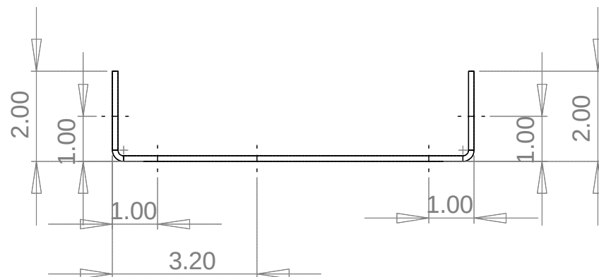
Profile - showing centers for 6" hole pattern.
