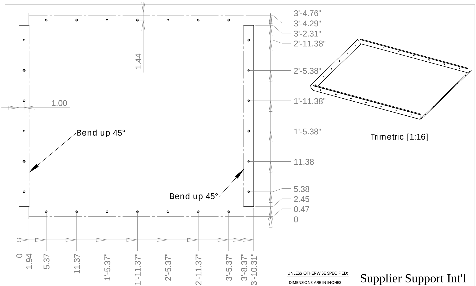
Flat Pattern
