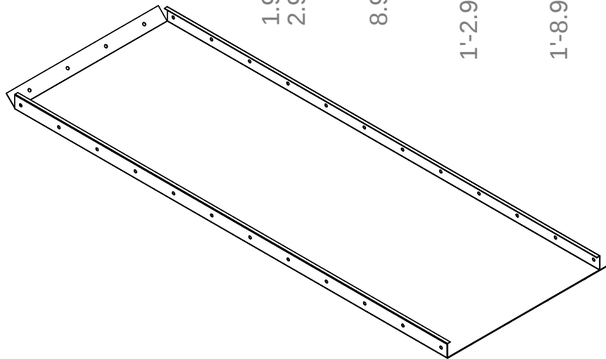
Isometric [1:10]
