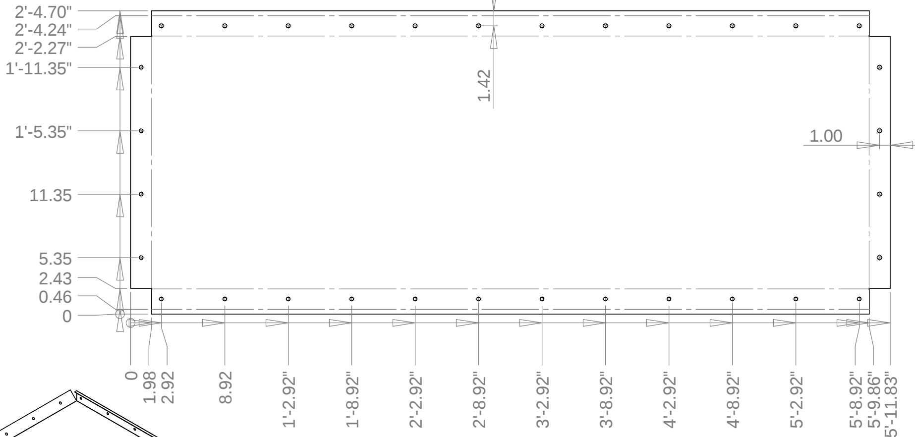
Flat Pattern
