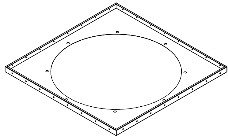
Isometric [1:18]
