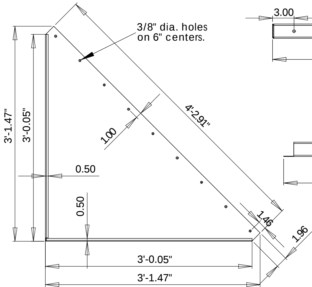
Bottom View
