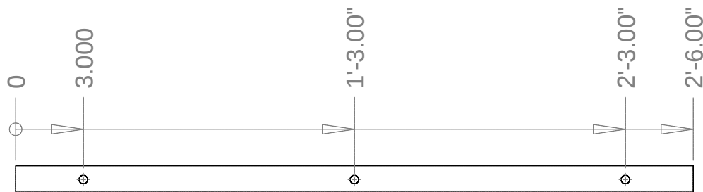
Front View [1:6] (bottom flange View)
